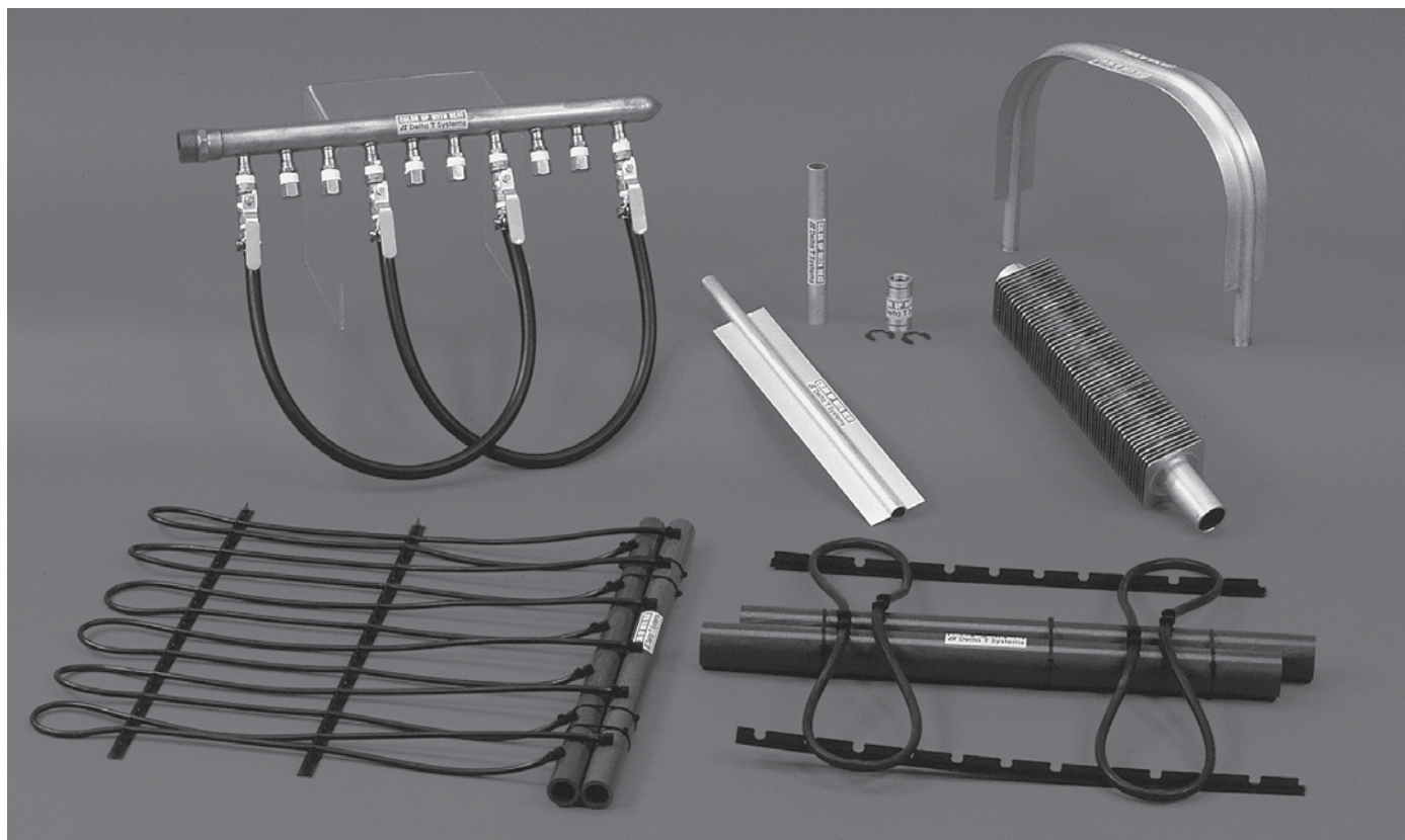
Delta-T Systems offers an array of hot water heating systems for virtually all types of growing needs.
